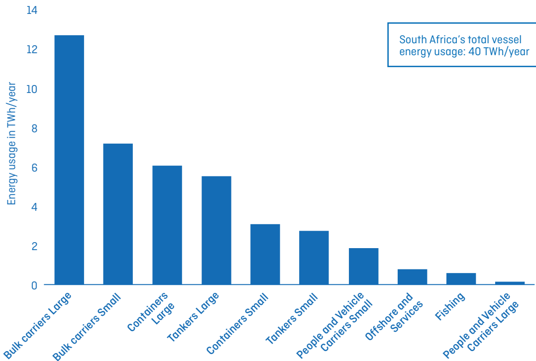
Exhibit 10: Energy usage by vessel category in 2018, based on energy required at departure.
